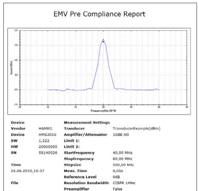
Abb. 8.3: EMV Report
