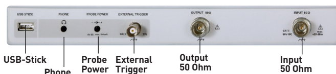
Fig. 10.1: Connections Front Panel
