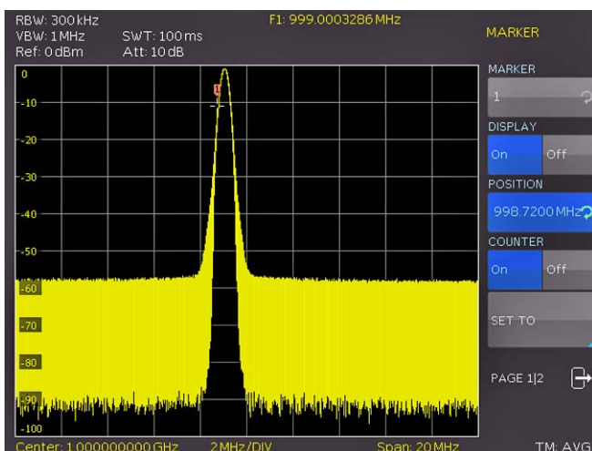
Fig. 6.7: Frequency counter
